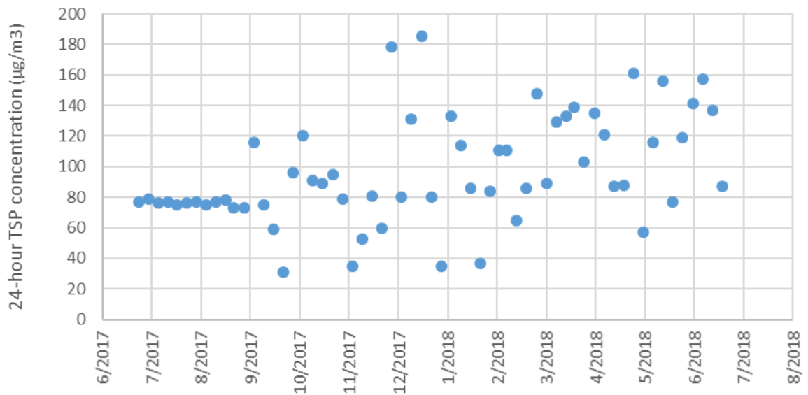
Measured 24-hour TSP Concentration ( \mu\text{g}/\text{m}^3 ) at DM2
