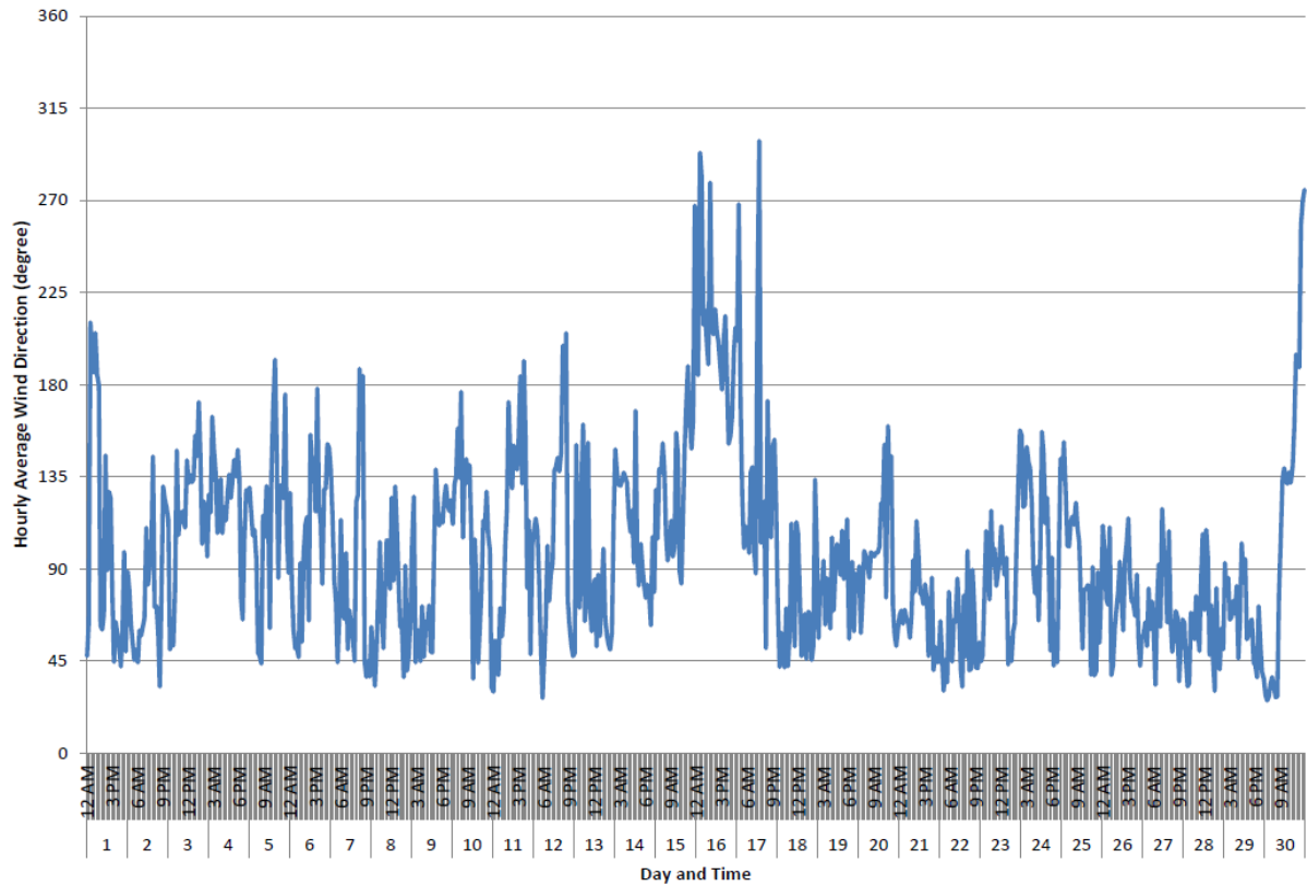
Hourly Average Wind Direction (degree) for November 2024
