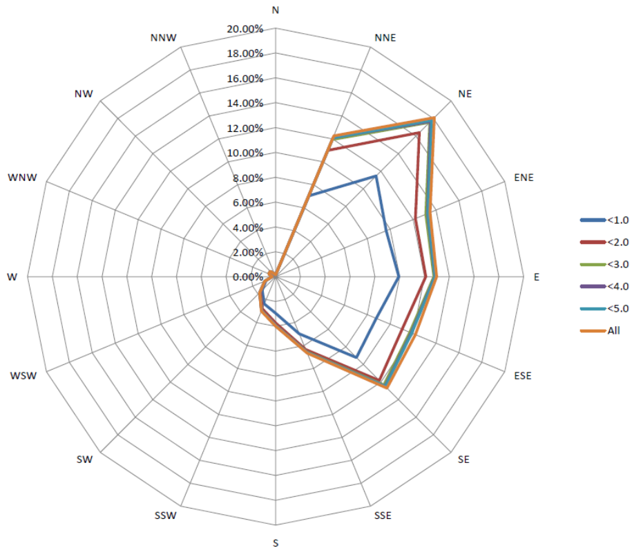
Wind Rose for November 2024
