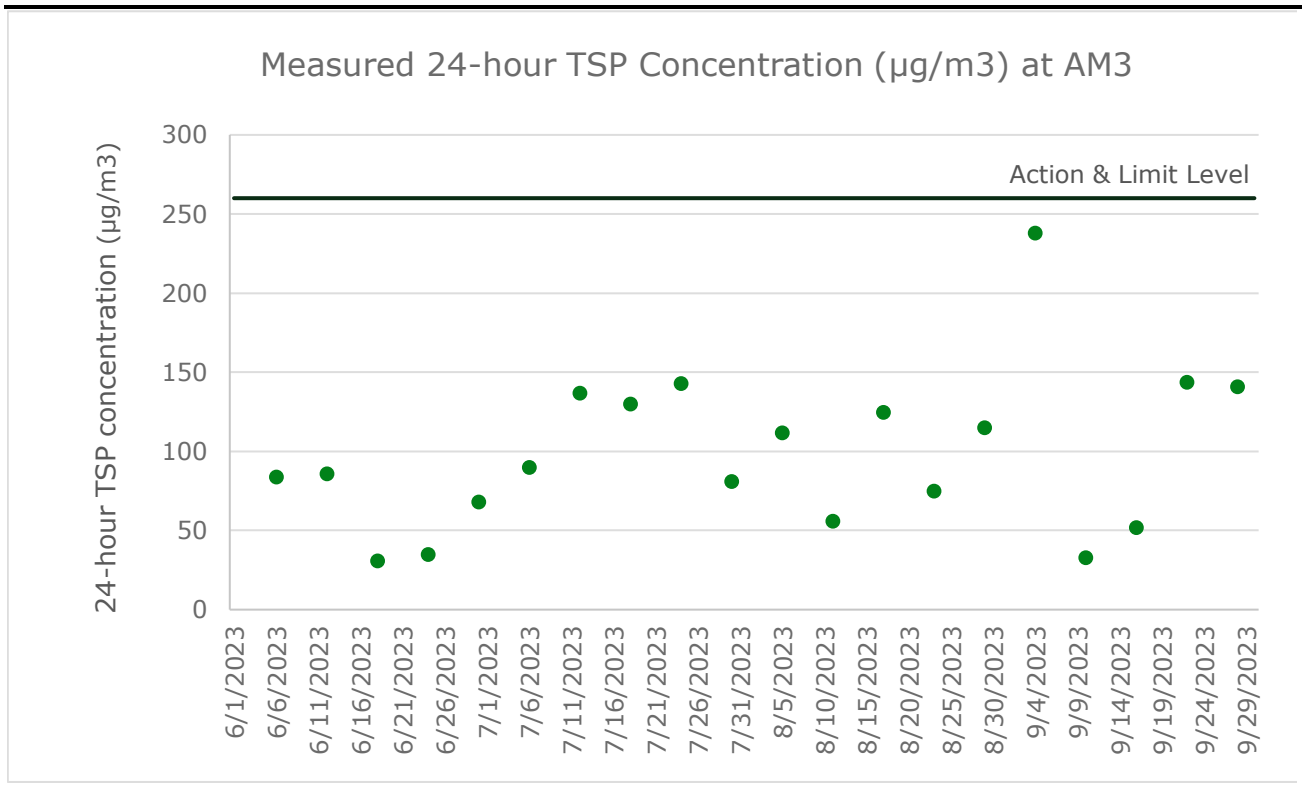
FIGURE D1.3 GRAPHICAL PRESENTATION FOR 24-HR TSP MONITORING AT AM3
