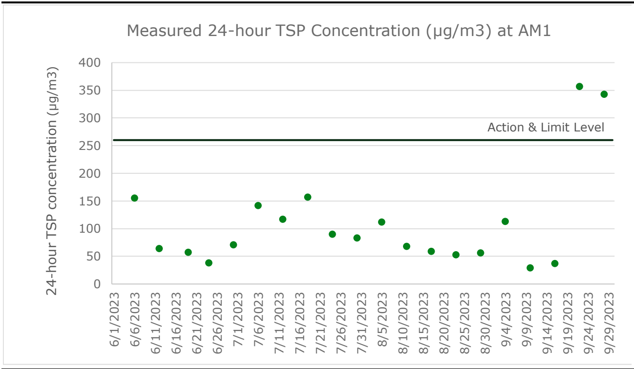
FIGURE D1.1 GRAPHICAL PRESENTATION FOR 24-HR TSP MONITORING AT AM1
