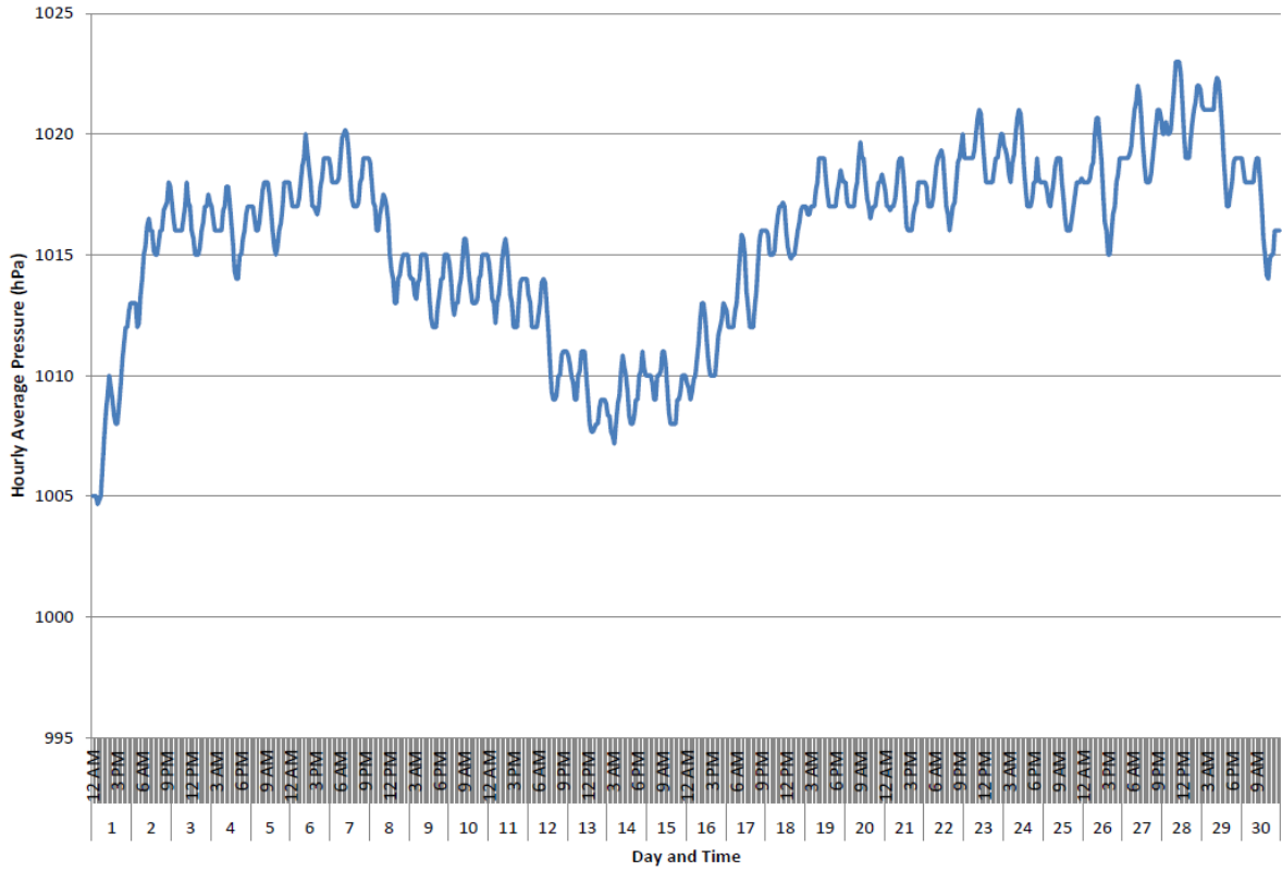
Hourly Average Pressure (hPa) for November 2024
