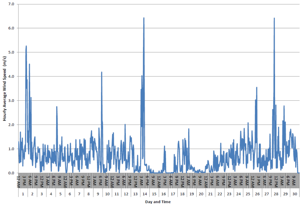
Hourly Average Wind Speed (m/s) for November 2024
