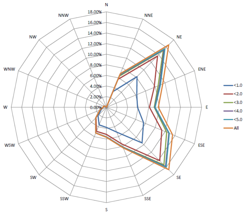
Wind Rose for Oct 2023
