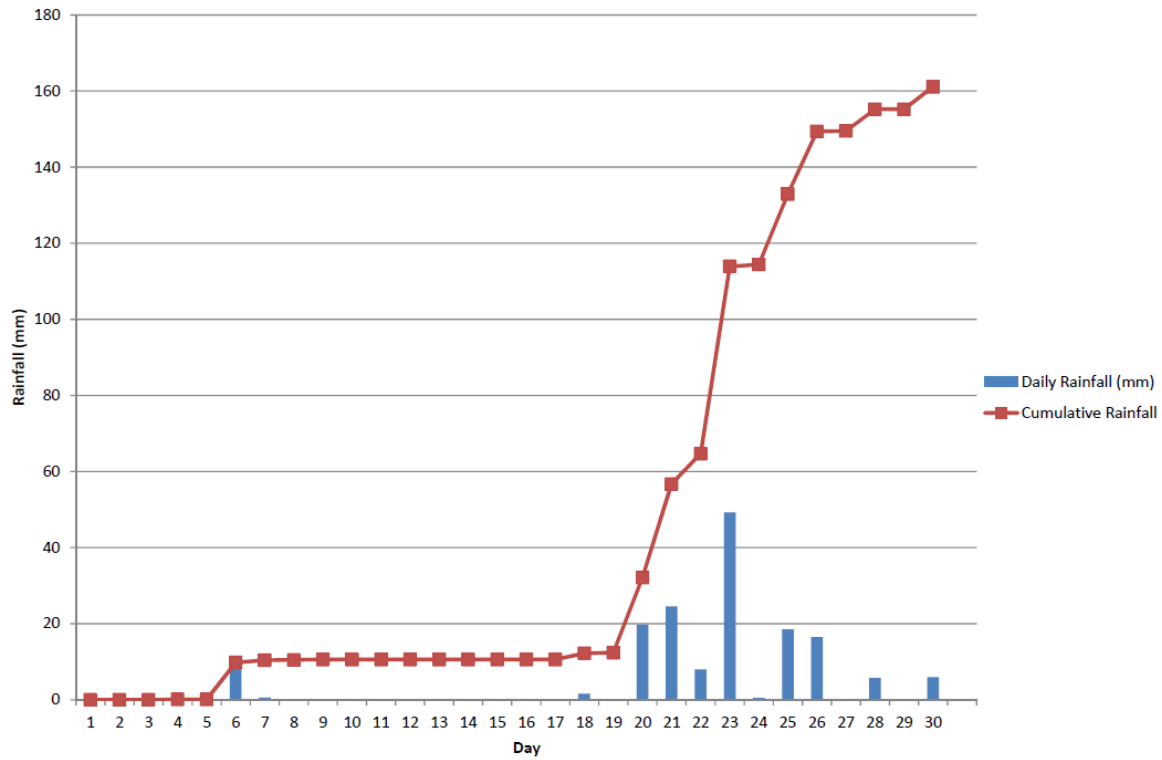
Daily and Cumulative Rainfall (mm) for April 2024
