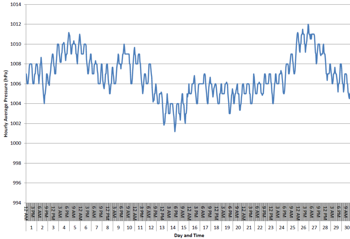
Hourly Average Pressure (hPa) for June 2024
