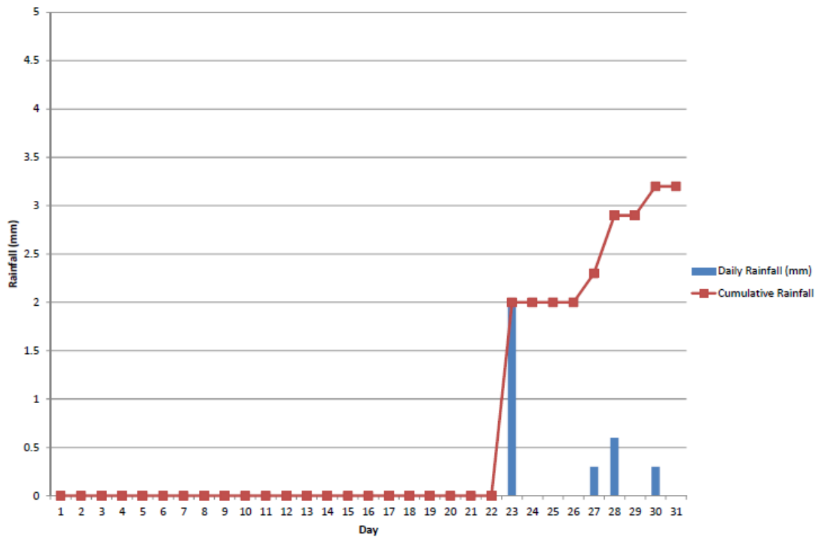
Daily and Cumulative Rainfall (mm) for January 2024
