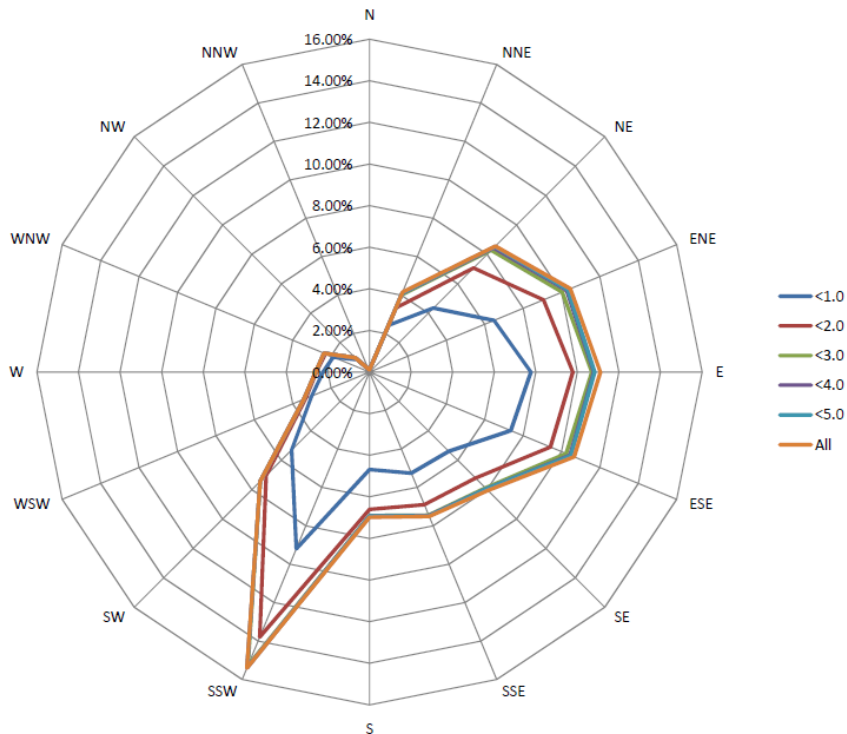
Wind Rose for March 2024
