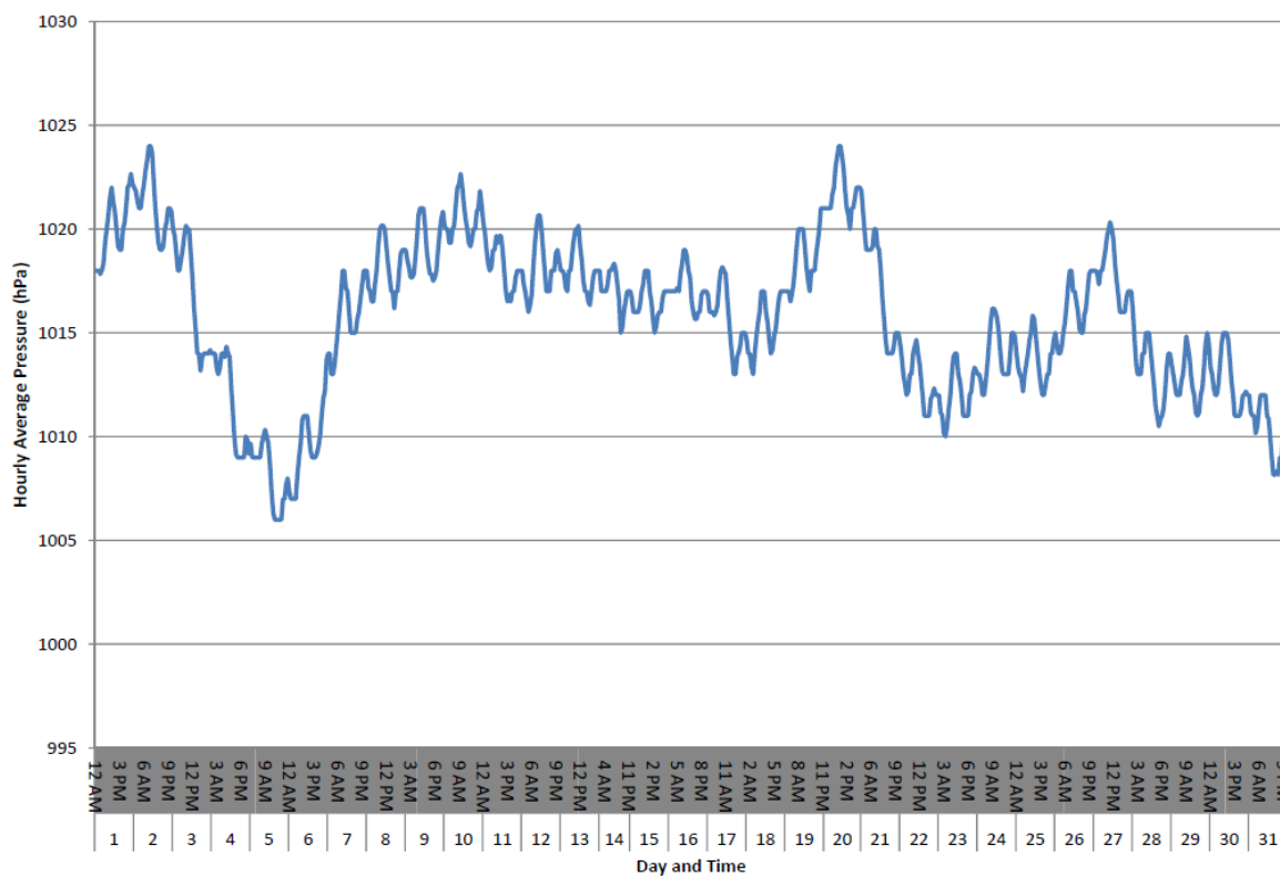
Hourly Average Pressure (hPa) for March 2024
