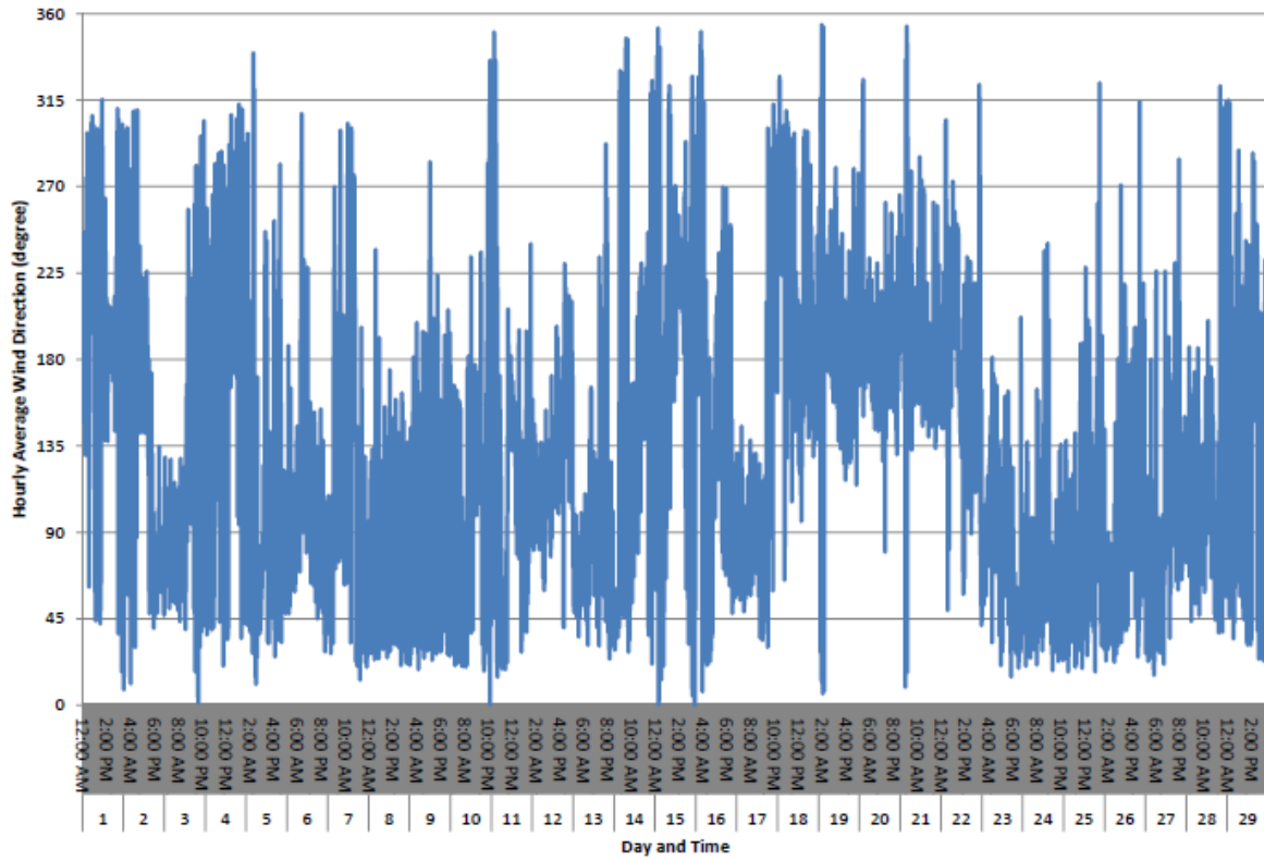
Hourly Average Wind Direction (degree) for February 2024
