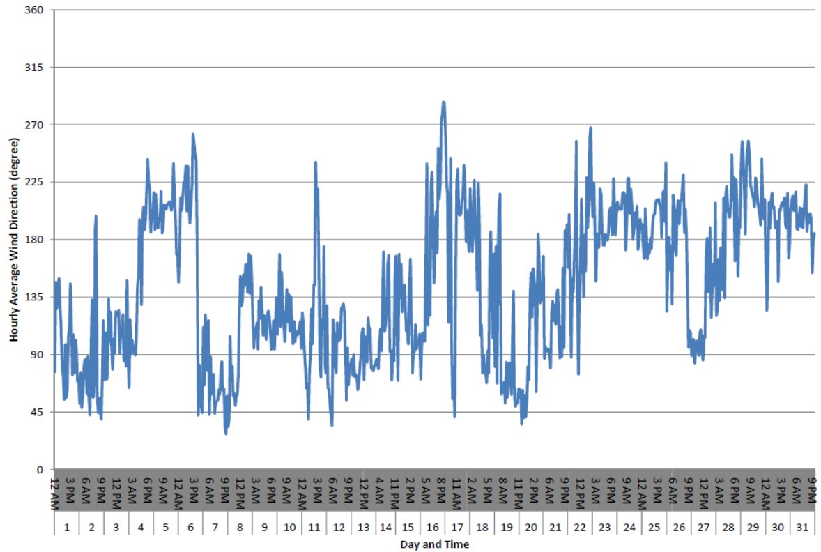
Hourly Average Wind Direction (degree) for March 2024
