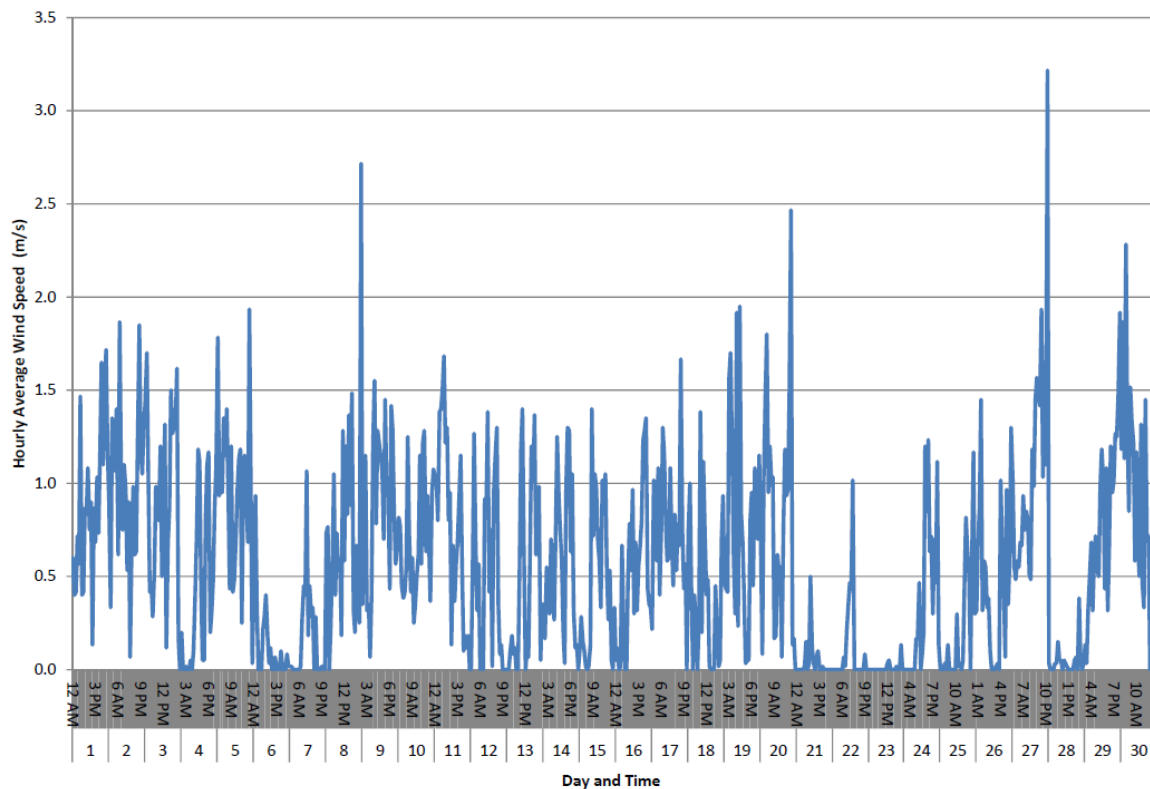
Hourly Average Wind Speed (m/s) for April 2024
