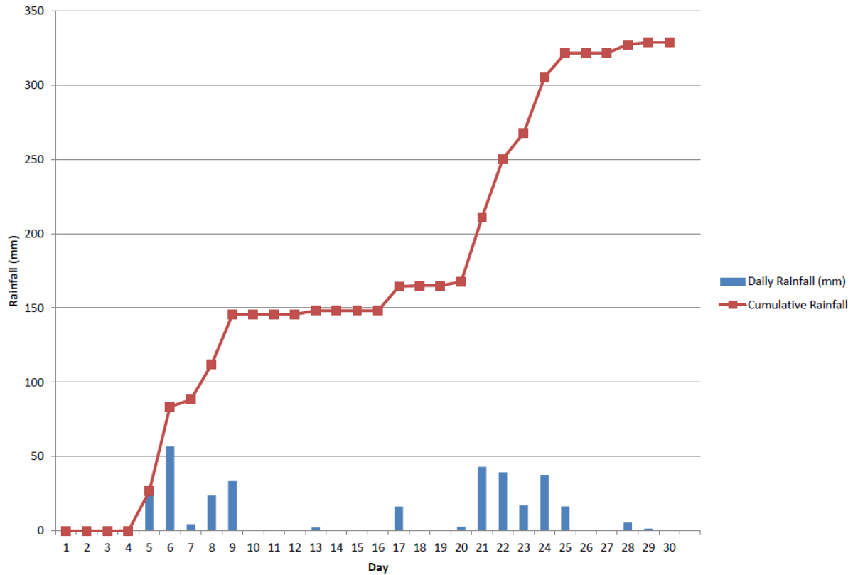
Daily and Cumulative Rainfall (mm) for September 2024
