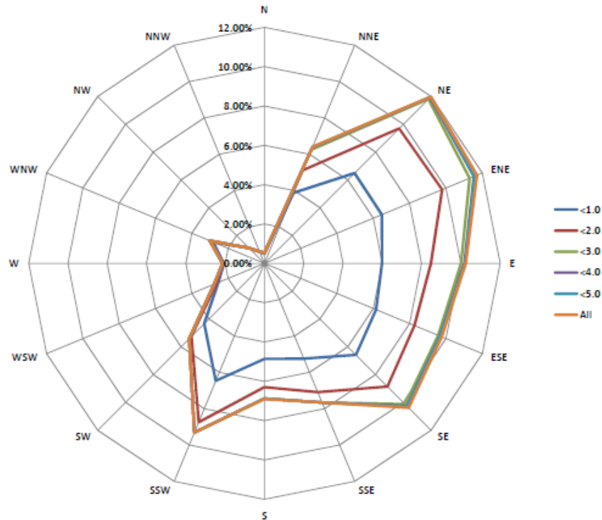
Wind Rose for February 2024
