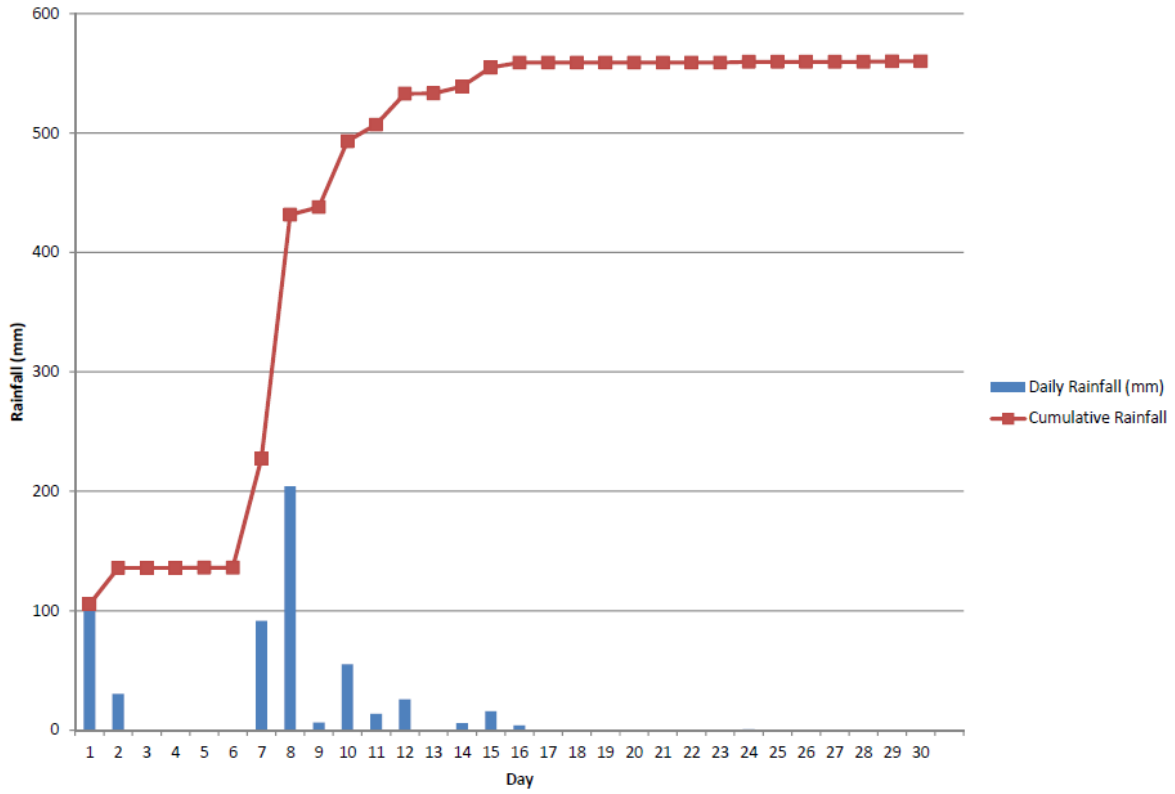
Daily and Cumulative Rainfall (mm) for September 2023
