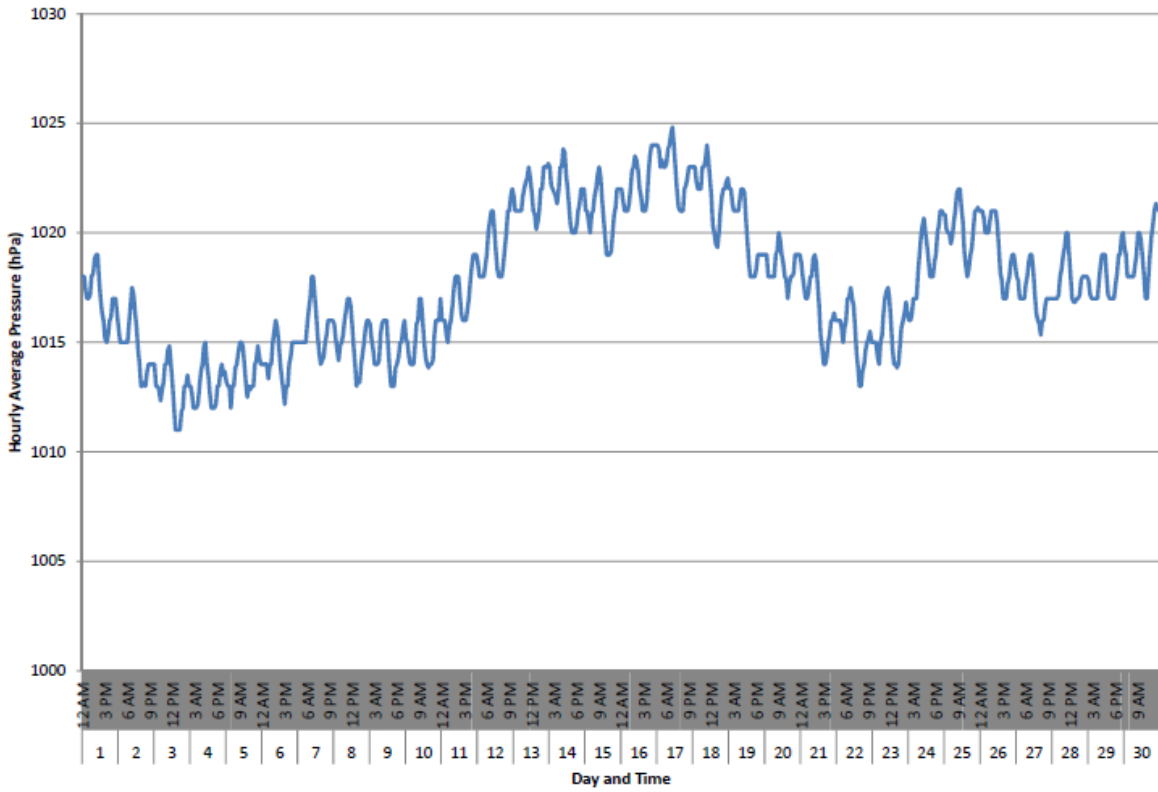
Hourly Average Pressure (hPa) for November 2023
