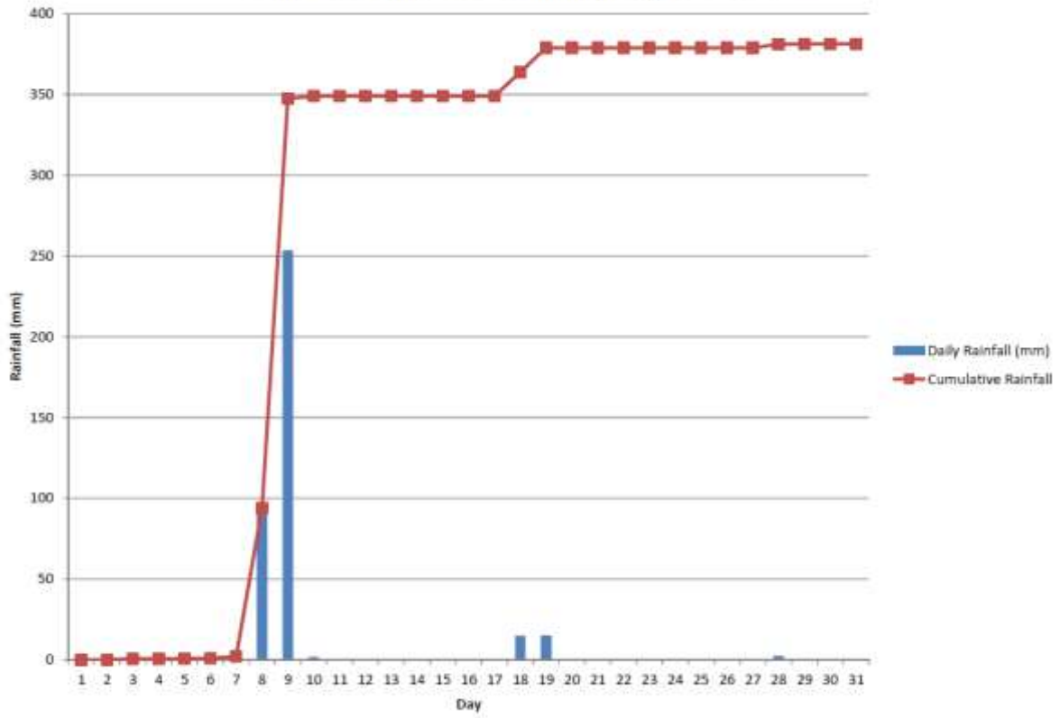
Daily and Cumulative Rainfall (mm) for Oct 2023
