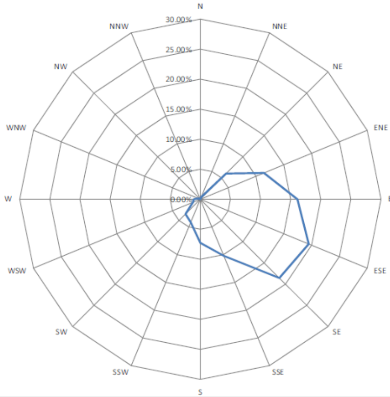
Wind Rose Diagram Percentage (December 2020)
